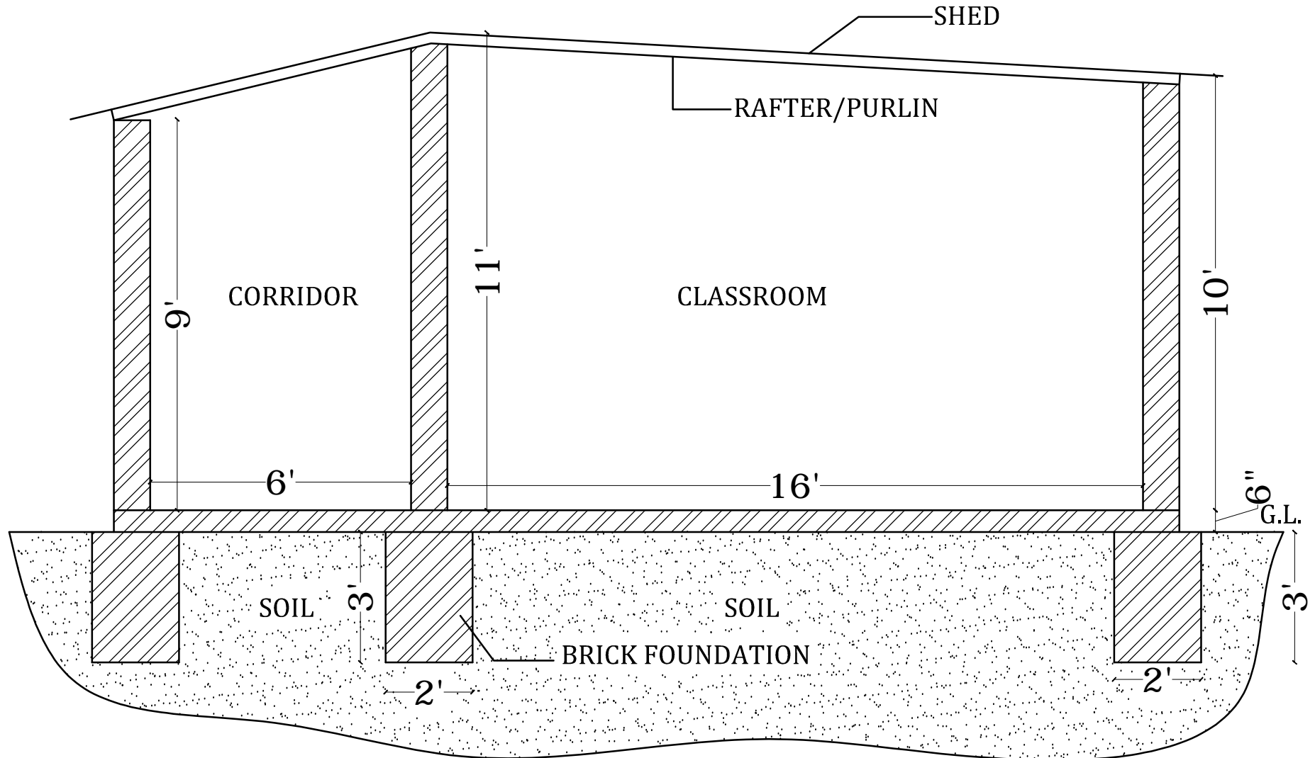
SECTION Y-Y'
